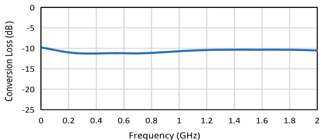
Conversion loss vs. Frequency
